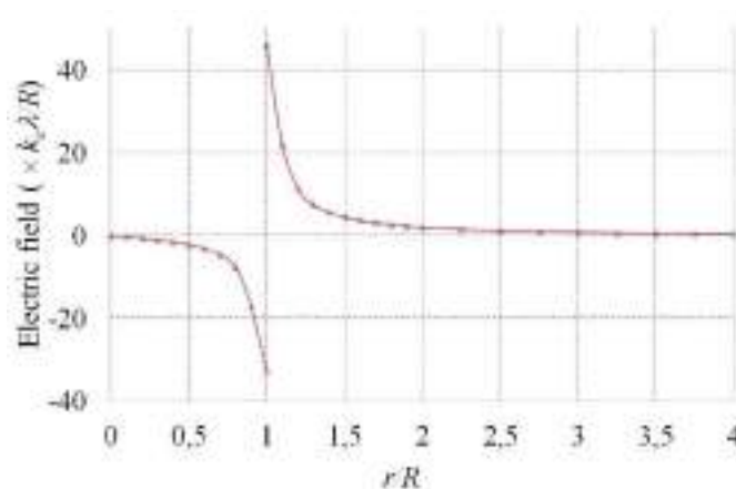
Figure 4. Electric field amplitude in the plane of a uniformly charged ring as a function of the relative radius a=r/R .
