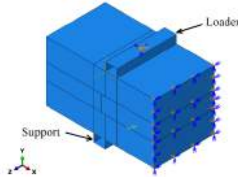
Figure 2. Numerical Specimen Testing Setup
