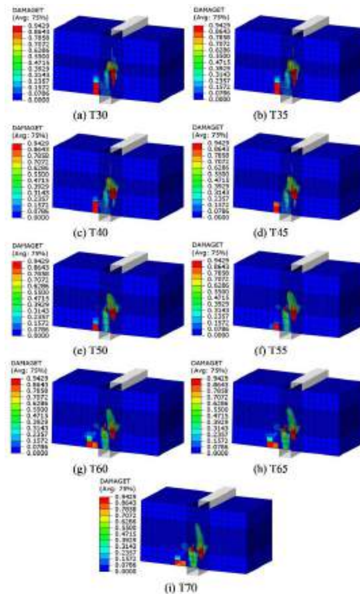
Figure 12. Damaget Contours for All Numerical Specimens
