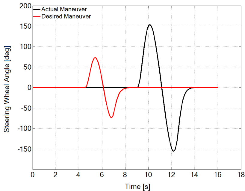
Figure 7. Steering Wheel Angle of the Remote Vehicle
