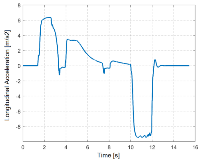
Figure 4. Simulation Scenario for the four-wheel model verification (vehicle longitudinal acceleration)
