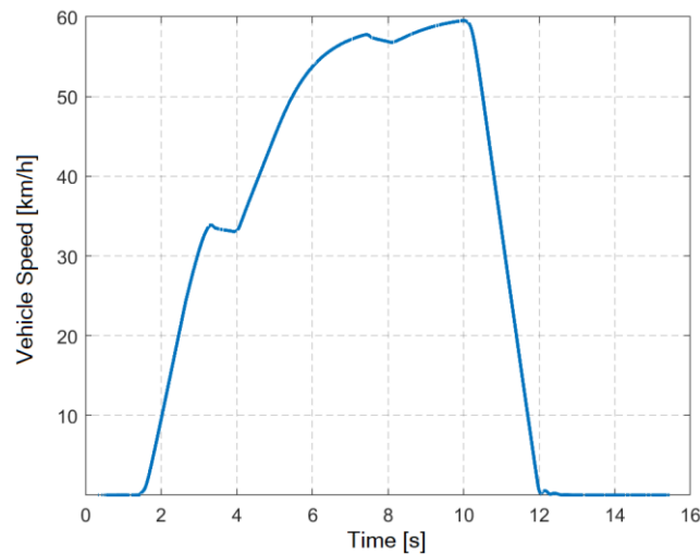
Figure 3. Simulation Scenario for the four-wheel model verification (vehicle speed)
