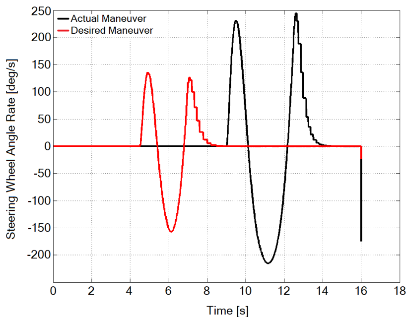
Figure 8. Steering Wheel Angle Rate of the Remote Vehicle
