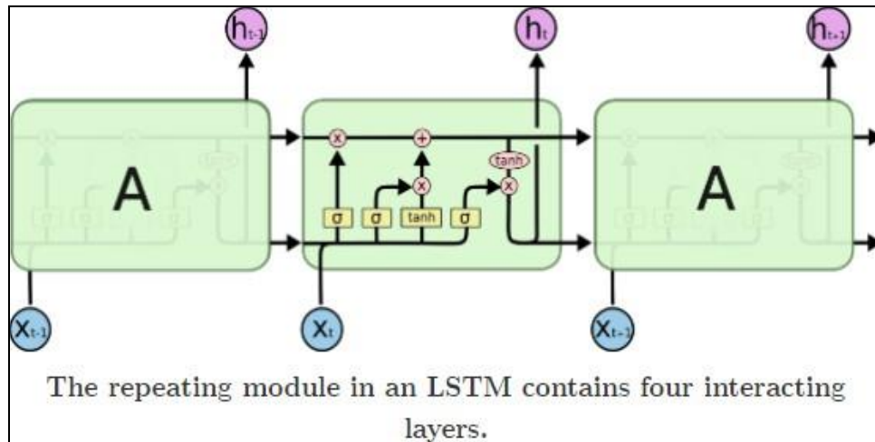
Figure 1. LSTM Layer Representation
