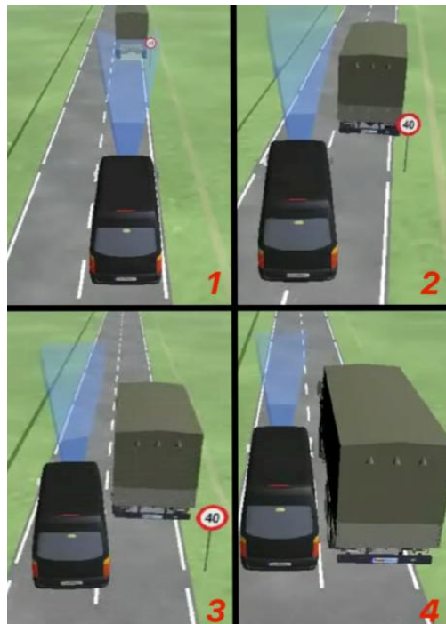
Figure 6. The strike avoidance maneuver of the TOV with the FLC
