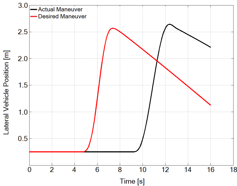
Figure 10. Lateral Vehicle Position of the Remote Vehicle
