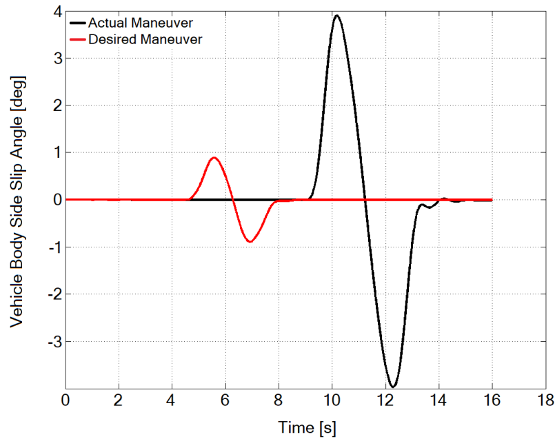
Figure 9. Vehicle Body Side Slip Angle of the Remote Vehicle
