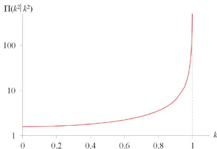
Figure 2. Complete elliptic integral of the third kind \Pi(k^2|k^2) vs. modulus k .
